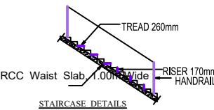
STAIRCASE DETAILS
