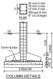
COLUMN DETAILS
