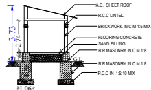
SECTION ON "AA"
