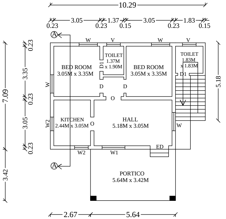
(Scale 1:100) (GROUND FLOOR PLAN) (Facing on East)
