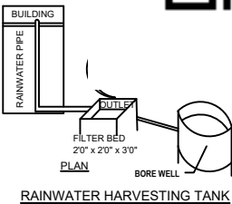
RAINWATER HARVESTING TANK
