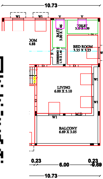
FIRST FLOOR PLAN ( Proposed Building )
