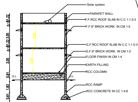
SECTION ON AA & BB
