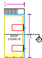
GROUND FLOOR PLAN SCALE 1:100
