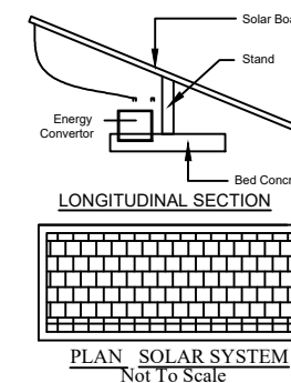
Width -3'-0"
