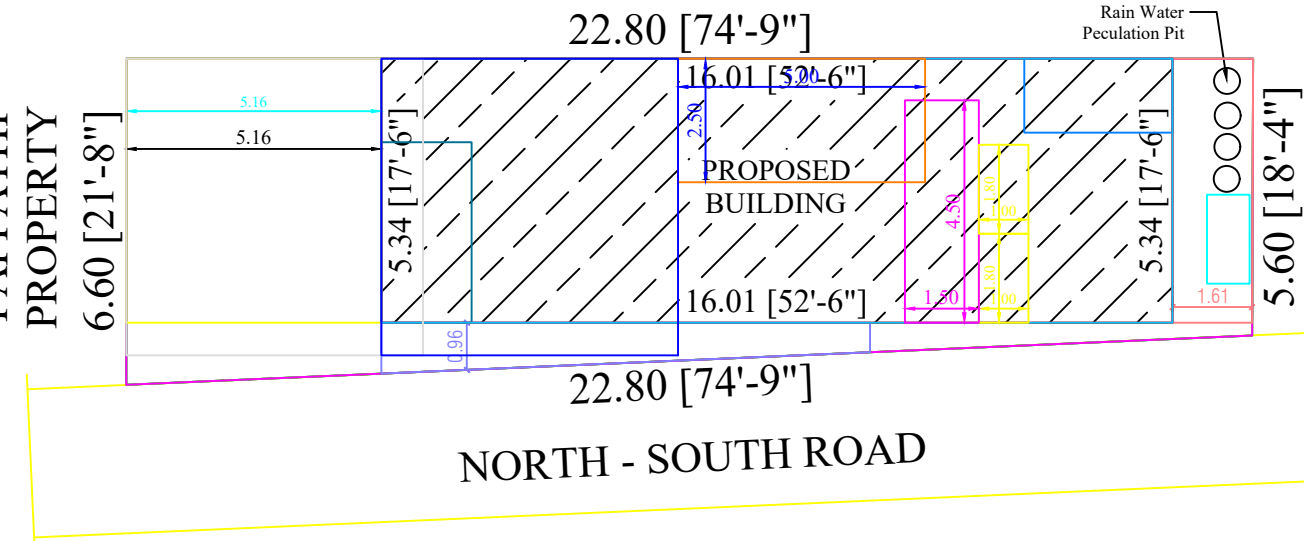
SITE PLAN
