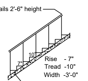
Width -3'-0"
