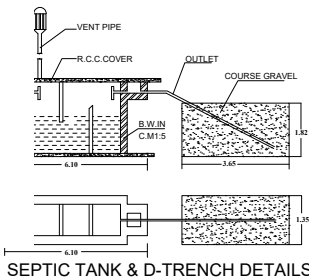
SEPTIC TANK & D-TRENCH DETAILS
