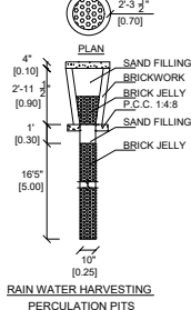
RAIN WATER HARVESTING PERCOLATION PITS
