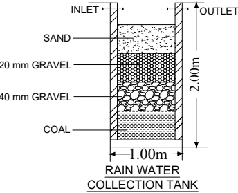
RAIN WATER COLLECTION TANK
