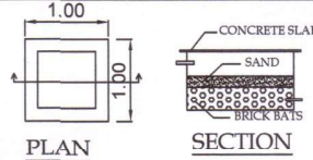
RAIN WATER HARVESTING TANK
