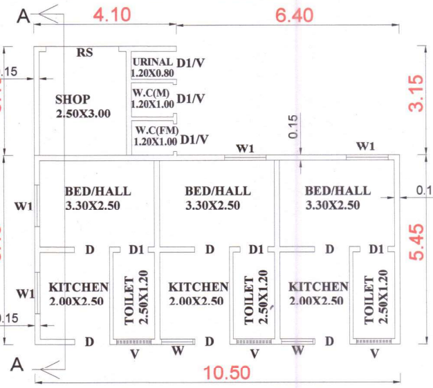
PLAN OF GROUND FLOOR
