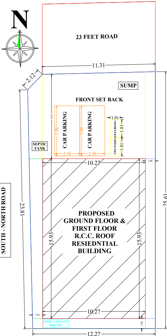
SITE PLAN
