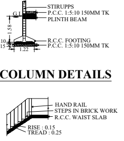
STAIR DETAILS
