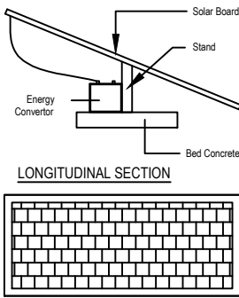
PLAN SOLAR SYSTEM Not To Scale
