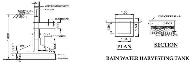
FOUNDATION DETAILS
