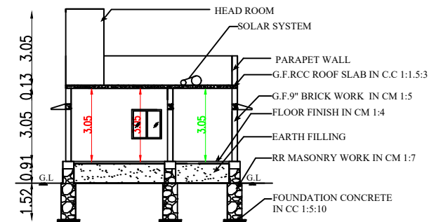
SECTION ON AA & BB
