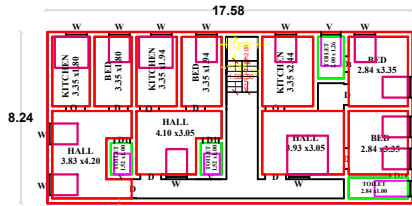
PROPOSED SECOND FLOOR
