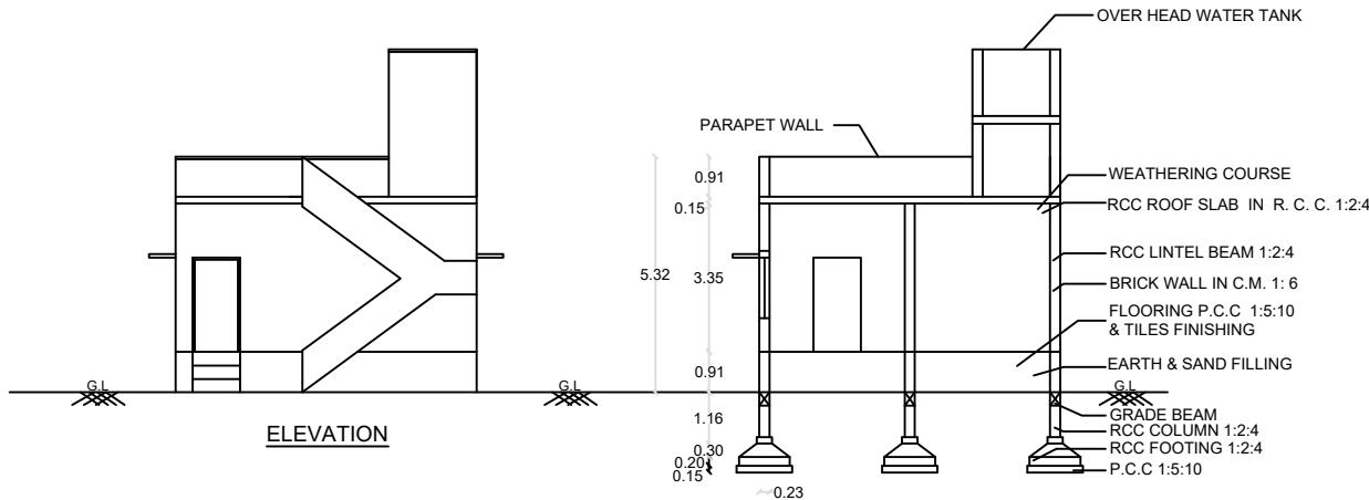
SECTION ON - XX
