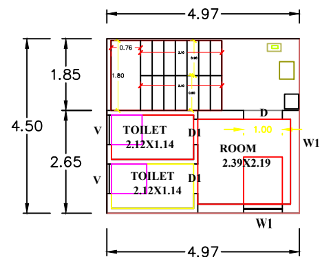
ADDL.PROPOSED FIRST FLOOR PLAN
