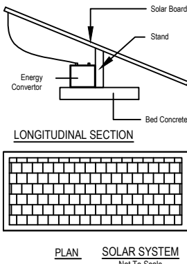
PLAN SOLAR SYSTEM Not To Scale
