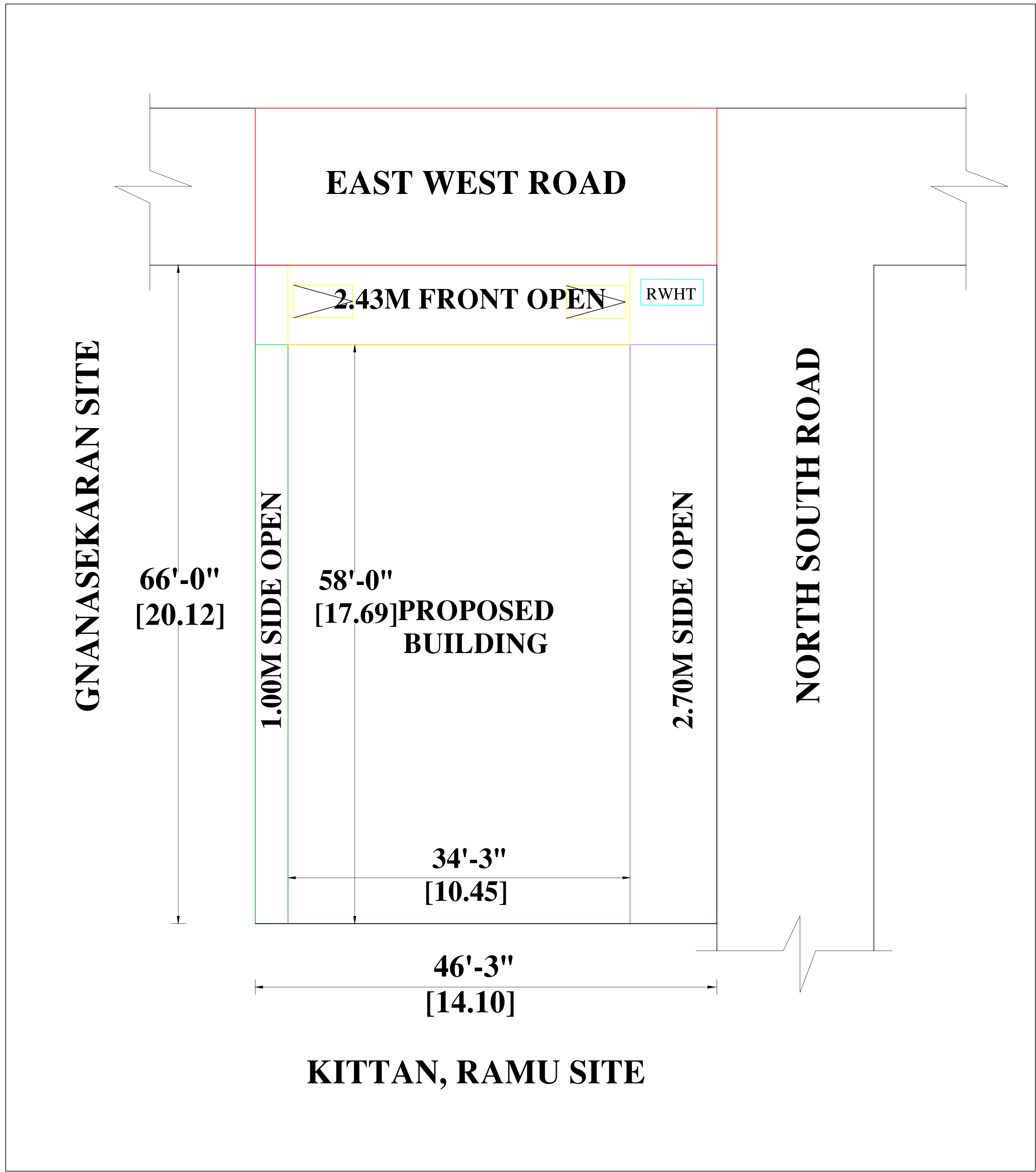
SITE PLAN
