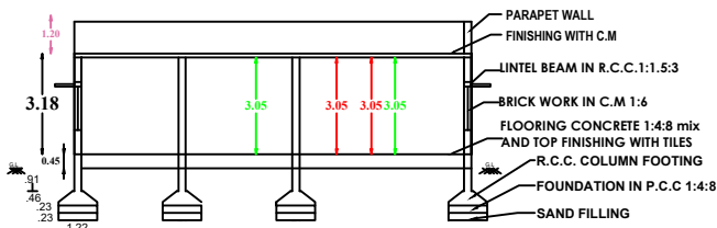
SECTION-AB
