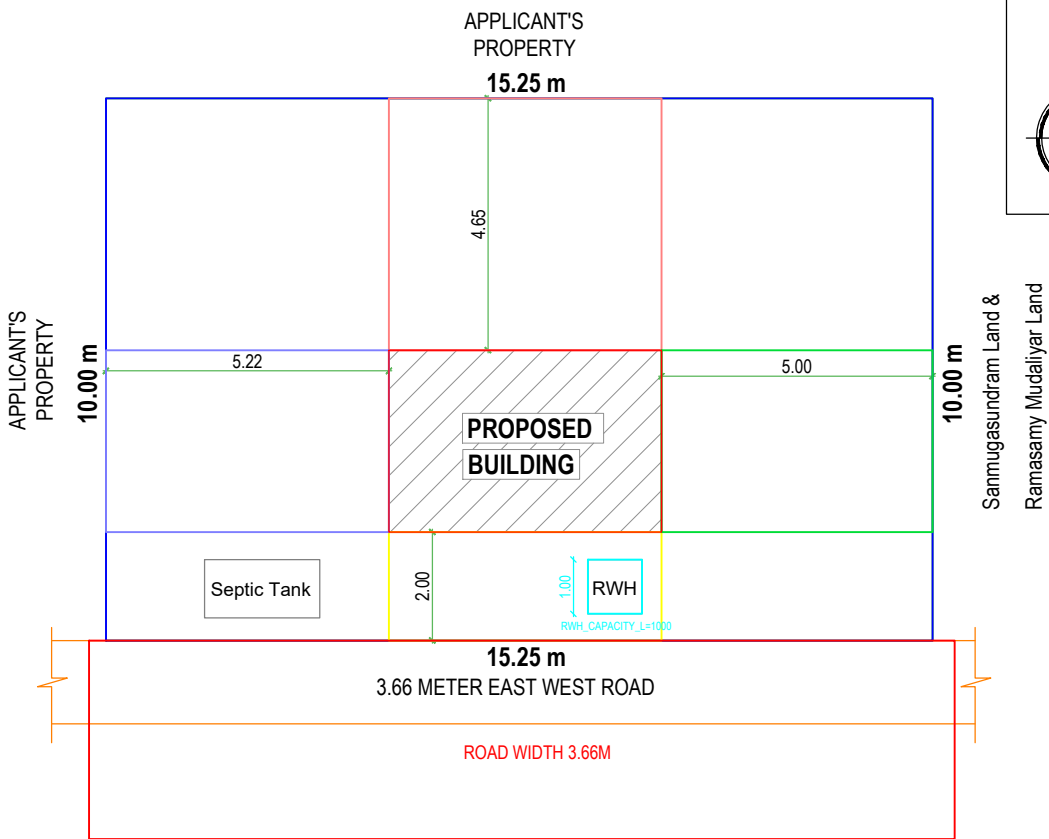
SITE PLAN
