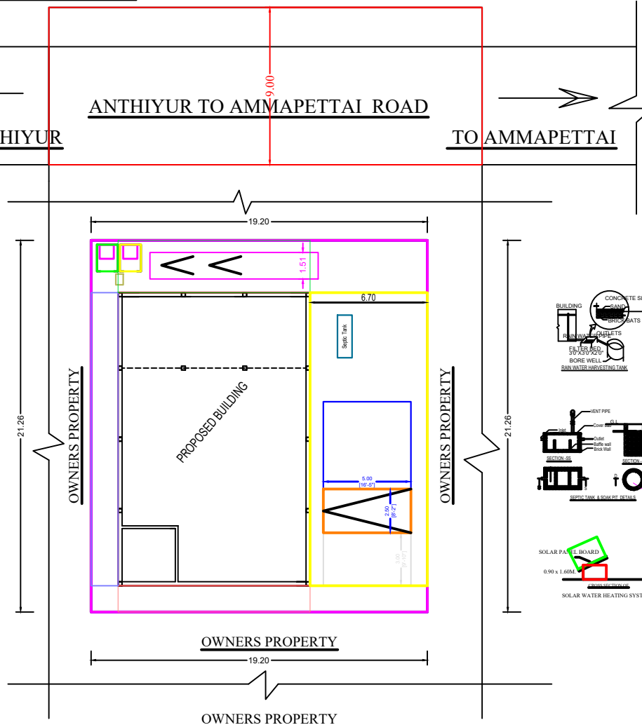
SITE PLAN
