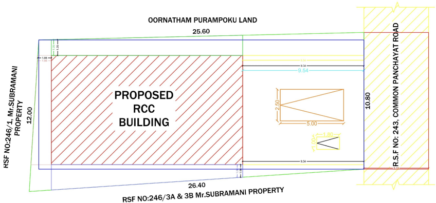
SITE PLAN
