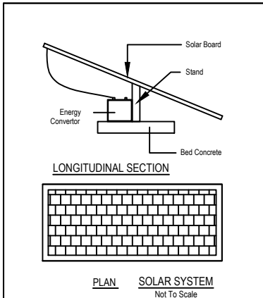
PLAN SOLAR SYSTEM Not To Scale
