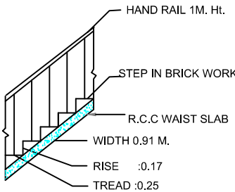
STAIR DETAIL
