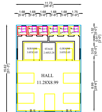
GROUND FLOOR PLAN (EAST)
