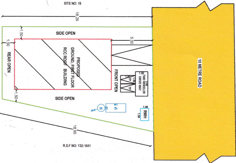
SITE PLAN
