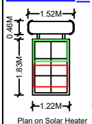
Plan on Solar Heater
