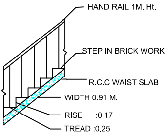
STAIR DETAIL
