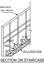
SECTION ON STAIRCASE
