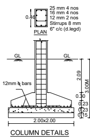
COLUMN DETAILS
