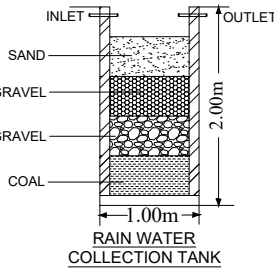
RAIN WATER COLLECTION TANK
