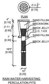
RAIN WATER HARVESTING PERCOLATION PITS
