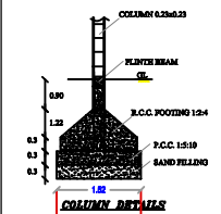
COLUMN DETAILS
