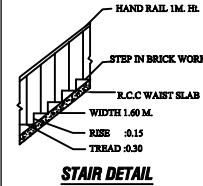
STAIR DETAIL
