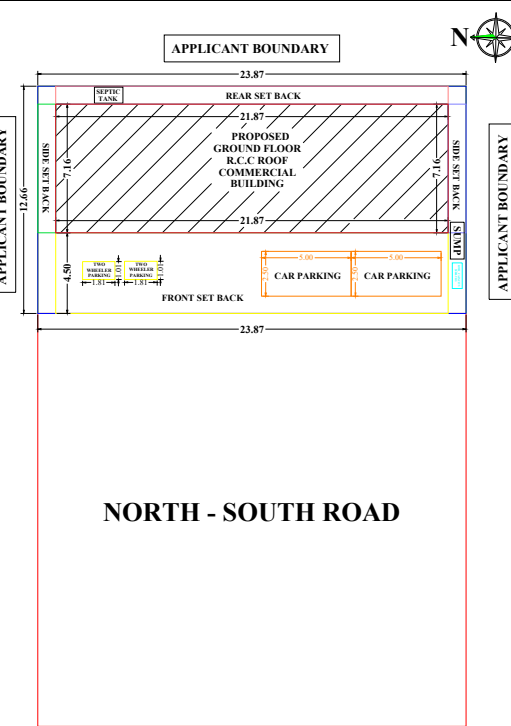
SITE PLAN
