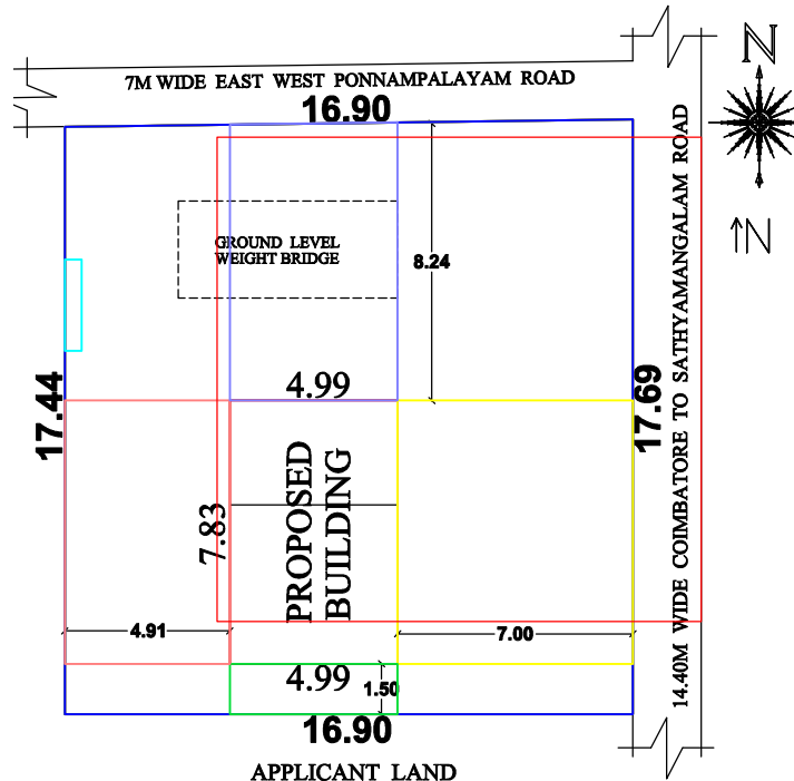
APPLICANT LAND
