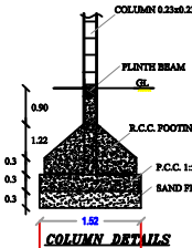
COLUMN DETAILS
