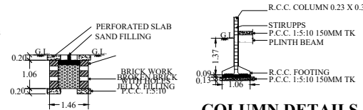
COLUMN DETAILS
