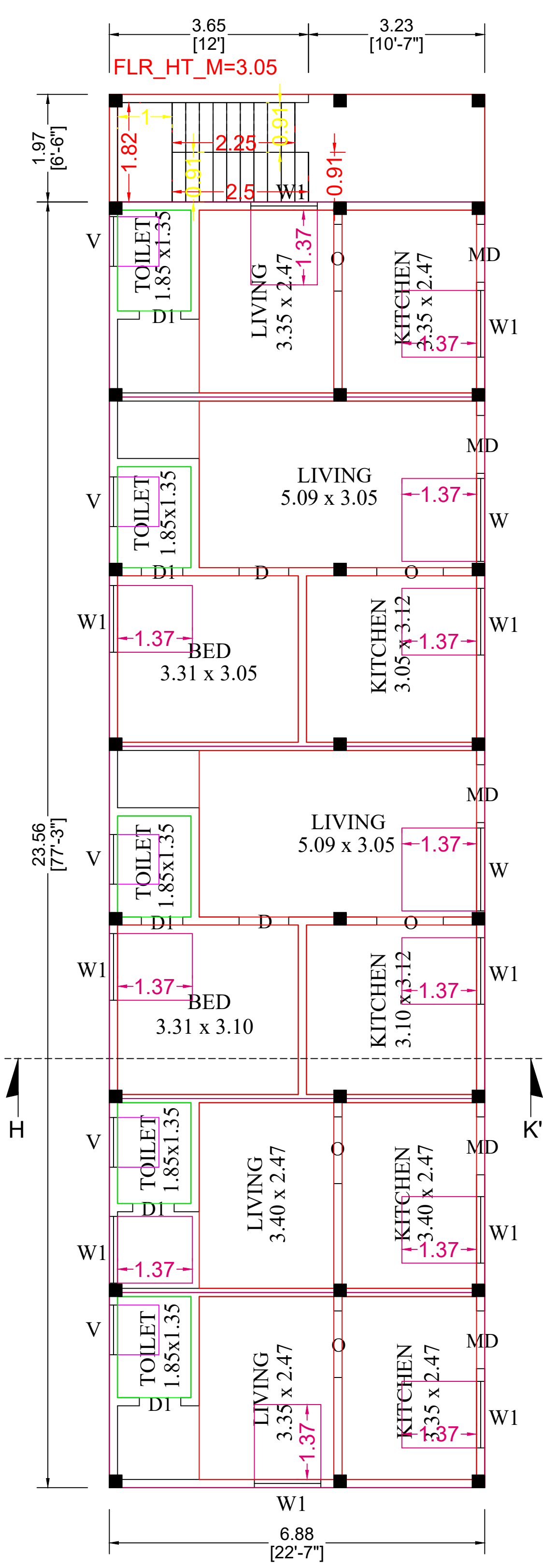
GROUND FLOOR
