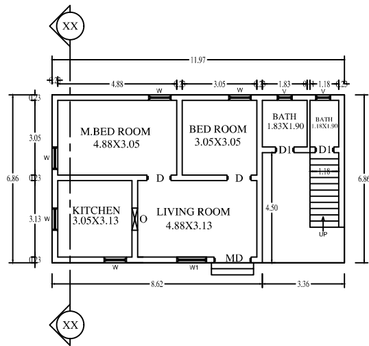
PROPOSED BUILDING OF GROUND FLOOR
