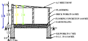
SECTION-AB
