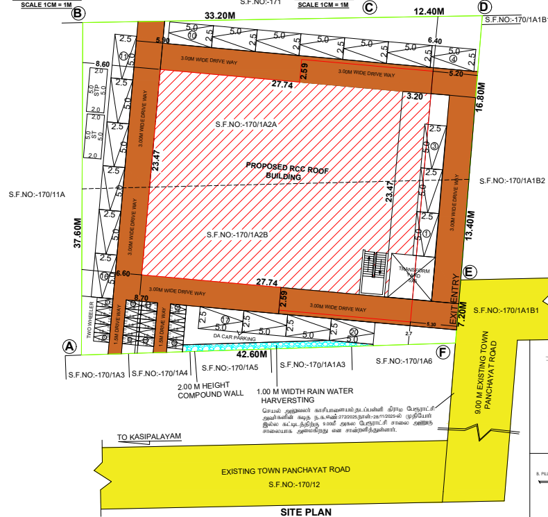
SITE PLAN
