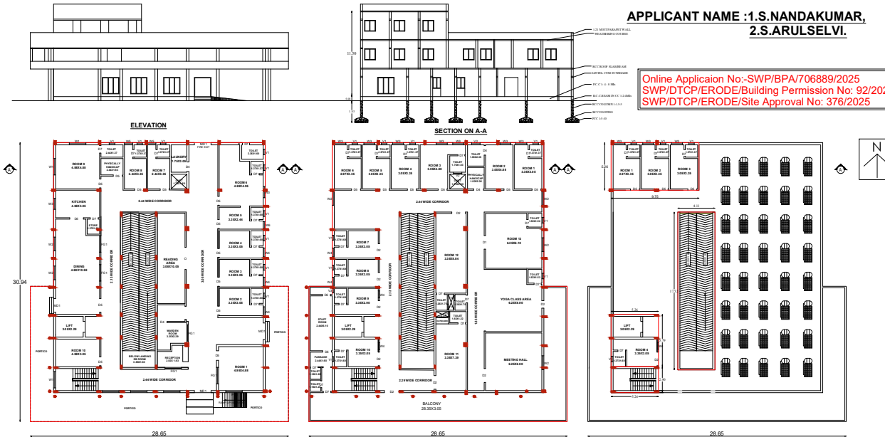
GROUND FLOOR PLAN SCALE 1CM = 1M
