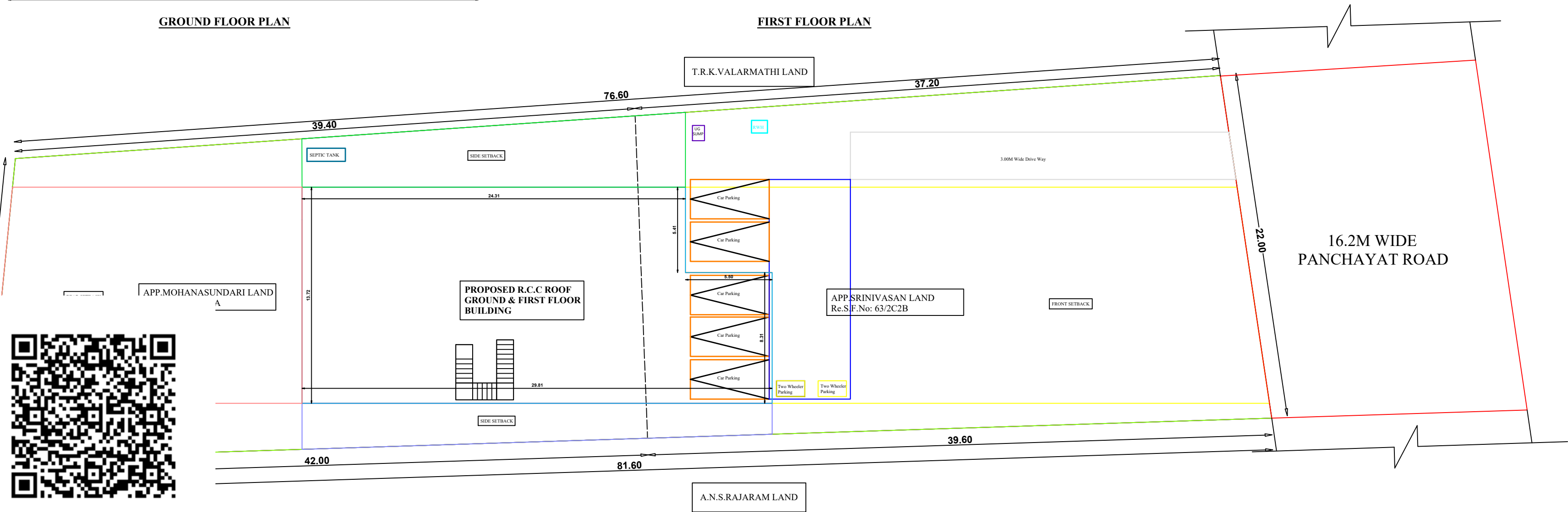
SITE PLAN
