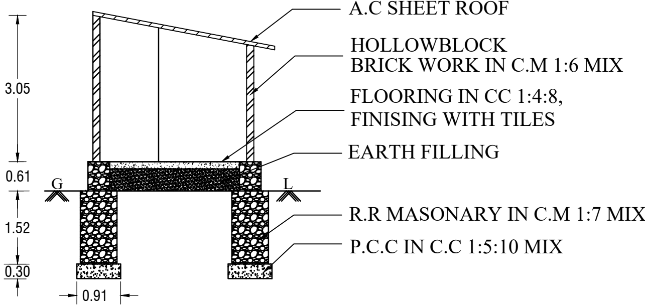
SECTION "A-B"
