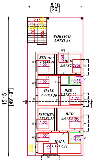
GROUND FLOOR PLAN (SCALE 1:100)
