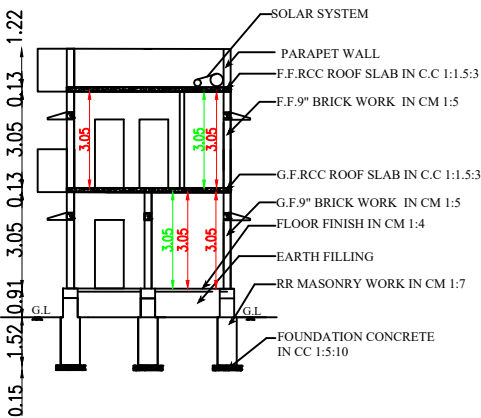
SECTION ON "AA & BB"
