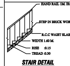
STAIR DETAIL
