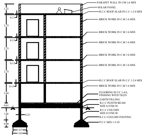
SECTION "A-B"
