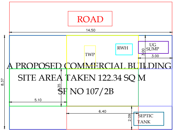
SF NO 107/2B OWN LAND
