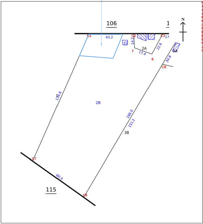
A PROPOSED COMMERCIAL BUILDING SITE AREA TAKEN 122.34 SQ M SF NO 107/2B
