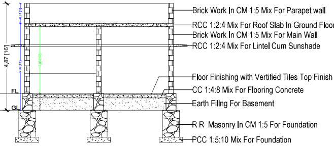
Building Section On "AA"
