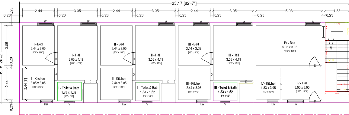
Building Plan - Ground Floor [Residential Building]
