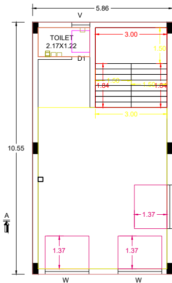
FIRST FLOOR PLAN FLR_HT_M=3.05
