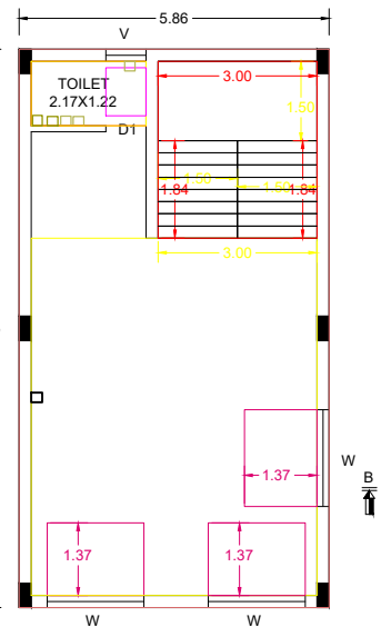
SECOND FLOOR PLAN FLR_HT_M=3.05
