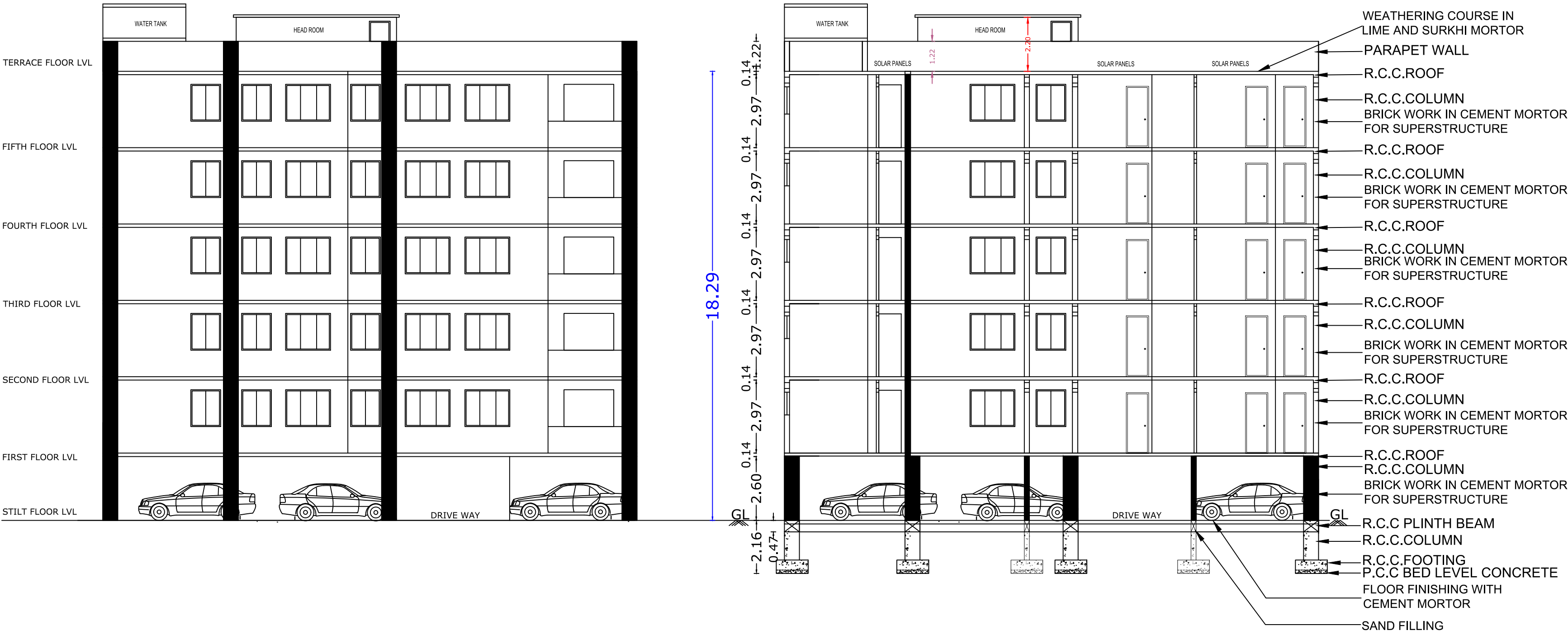
FRONT ELEVATION
