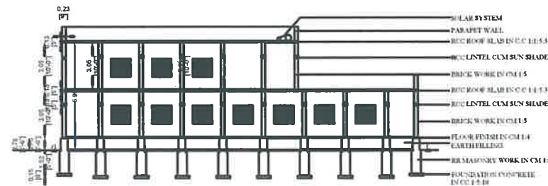
SECTION "AA","BB"
