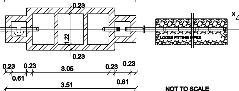
SEPTIC TANK & DISPERSION TRINCH
